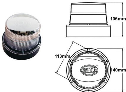
Model K-LED 360 E Fixed multi-voltage amber LEDs clear lens
