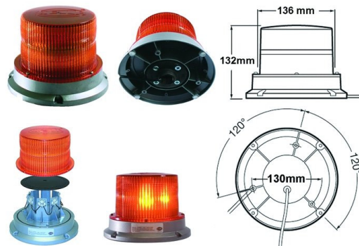
Model K-LED 450 Fixed multi-voltage amber LEDs amber lens
